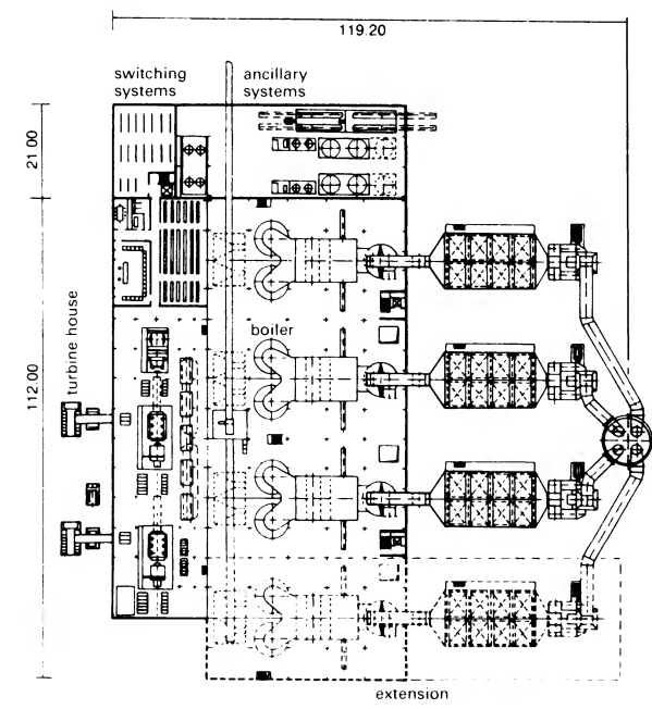
4 Plan of power station with fluidised bed firing
